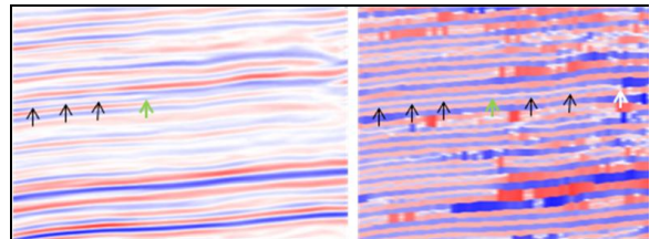
Figure 3 The effect of the Terrace attribute (right) on the input reflectivity data (left). The black arrows highlight a peak event (red) which pinches out in the original data at the location of the green arrow. In the Terrace attribute the same peak is a continuous event much further along the section until the position of the white arrow.
