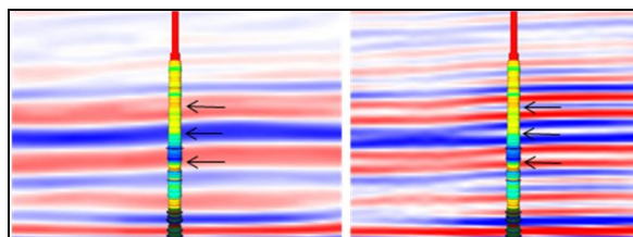
Figure 5 The seismic reflectivity data before (left) and after (right) application of the Spectral Enhancement workflow. The log data shows the gamma ray response with red indicating low gamma ray and blue indicating high gamma ray. The black arrows indicate areas where reflectors are only visible after the Spectral Enhancement and which correspond to a change in the gamma ray response.
