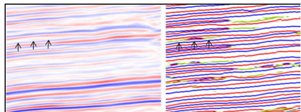
Figure 4 The Bedform attribute (right) which skeletonises the peaks and troughs (red and blue) and identifies unresolved events (green lineations) by incorporating the instantaneous frequency anomalies. The circles show areas where there appear to be pinch outs, but the negative frequencies help extend the reflectors. This could be used to map locations where the beds reach a critical thickness (tuning).
